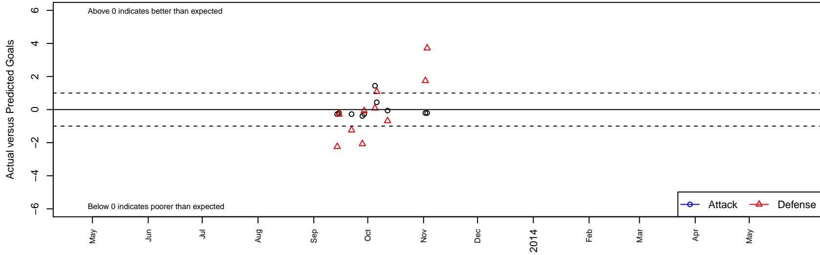
The Academy Cads G00 Dots are actual minus expected GF (blue circles) and GA (red triangles). Blue line is smoothed change in attack strength. Red is smoothed change in defense strength.
